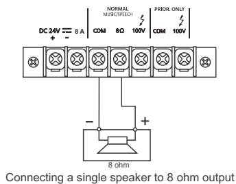
Connecting a single speaker to 8 ohm output
